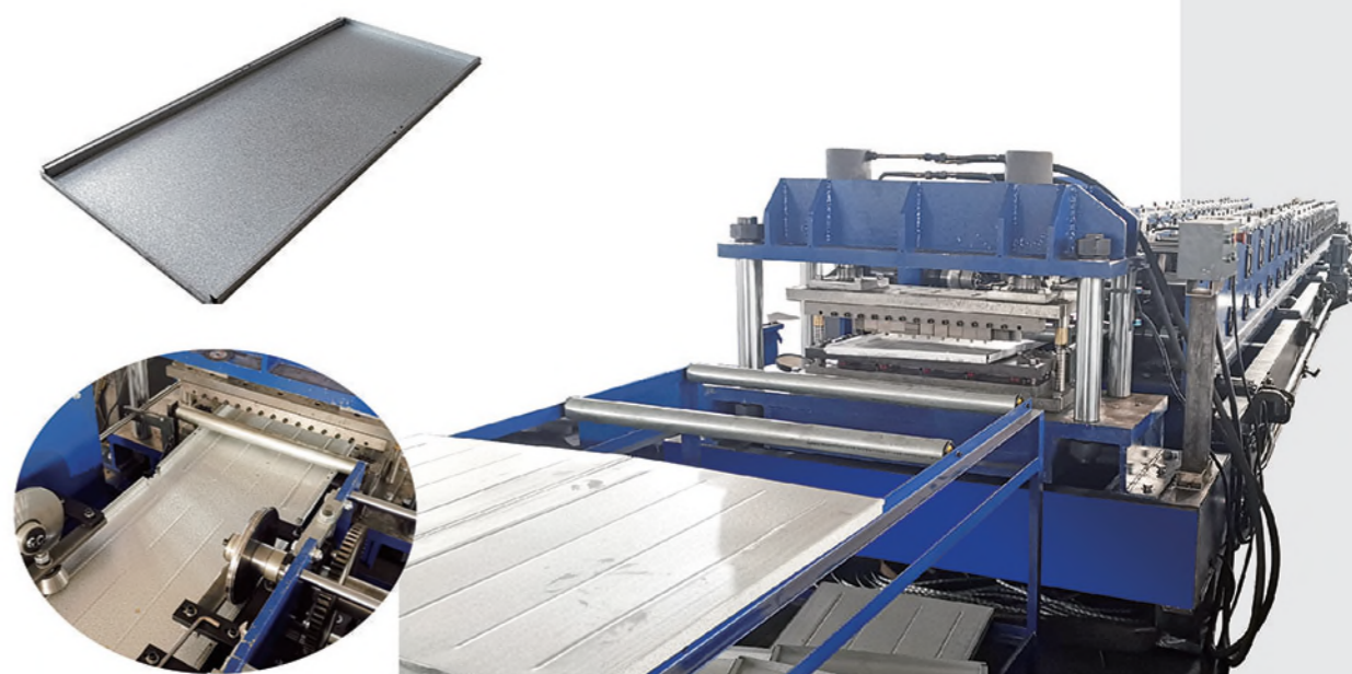
货架承板冷弯成型生产线 Shelf/Rack panel roll forming machine
