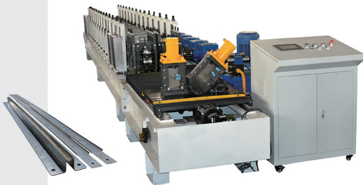
轻钢龙骨压型机 Stud-Track roll forming machine
