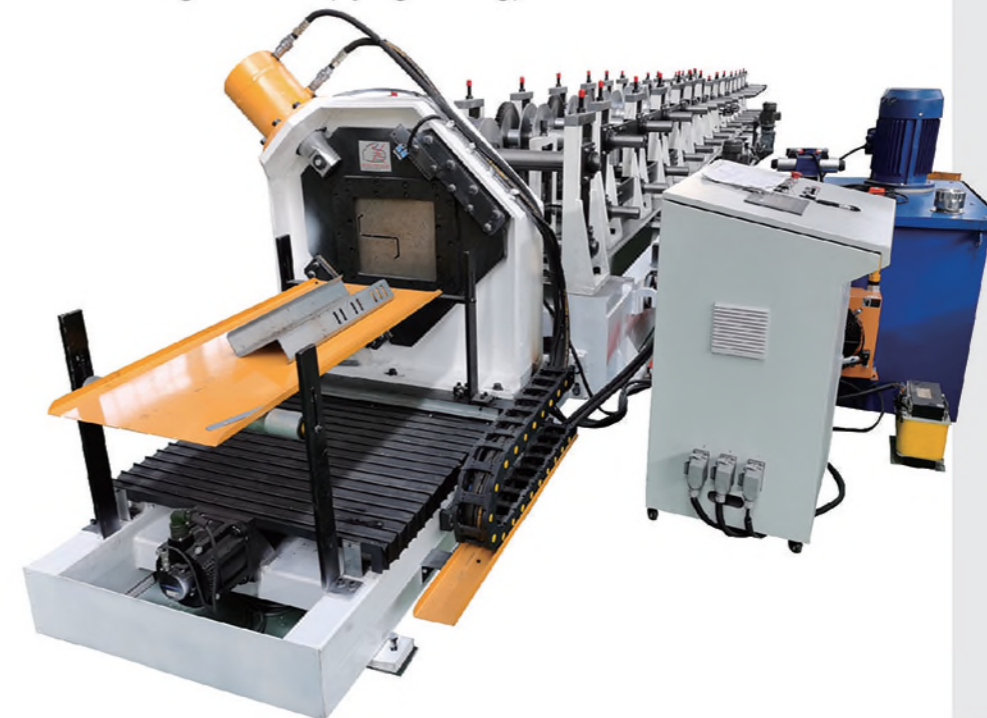
C/Z 互换成型机(跟踪剪切) C/Z purlin roll forming machine(flying cutting)
