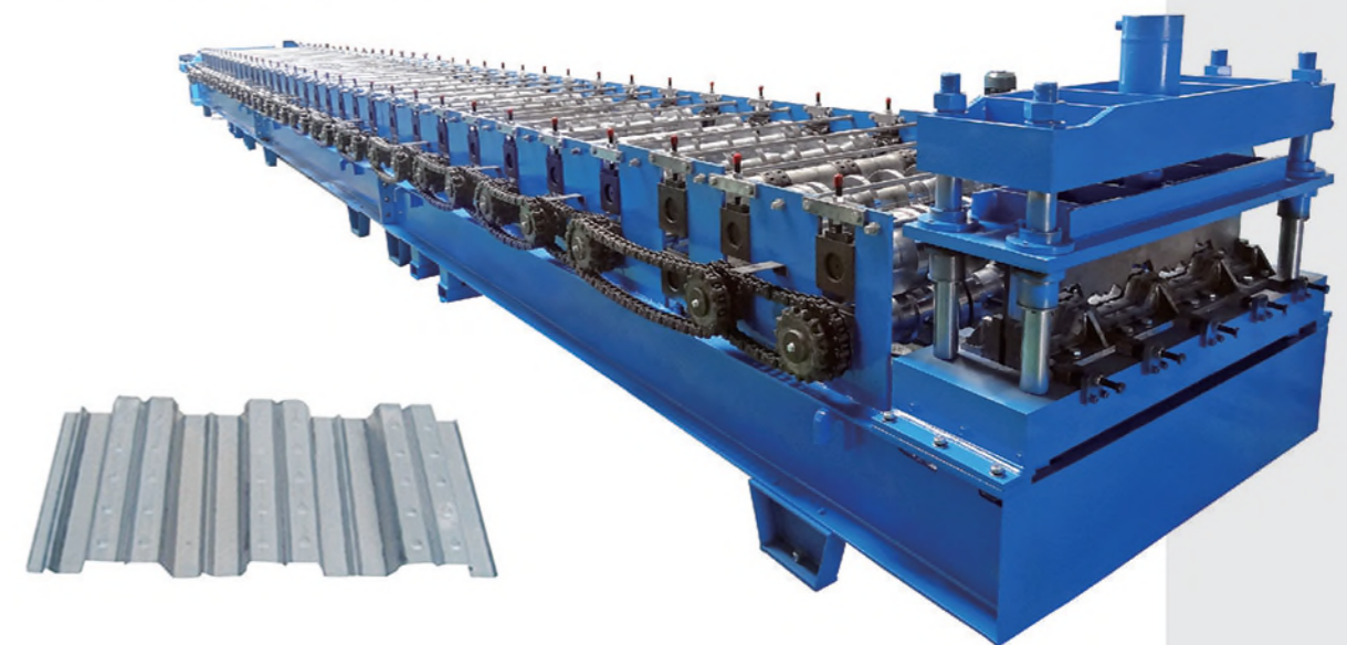
楼承板成型机 Floor Deck roll forming machine
