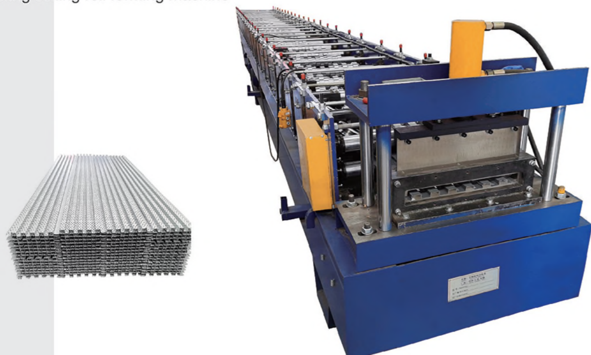
屋面吊顶扣板机 Roofing ceiling roll forming machine
