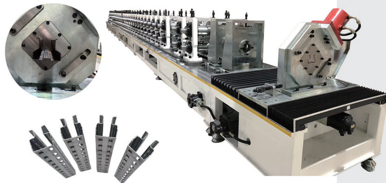
货架冷弯成型生产线 Shelf/Rack roll forming machine
